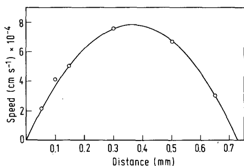
Fig. 3. Dependence of the vertical velocity of the chamber depth along the y -axis. The full line shows the parabolic curve that fits best to the measured points. Polystyrene beads of 8\text{ }\mu\text{m} diameter in 0.1\text{ M NaCl} , E-field 7.6\text{ V/cm} , B-field 52 \times 10^{-4}\text{ T}
