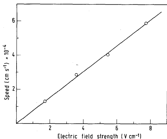
Fig. 7. Vertical velocity versus E-field. Polystyrene beads of 8\ \mu\text{m} diameter in 0.1\ \text{M NaCl} , B-field 52 \times 10^{-4}\ \text{T}
