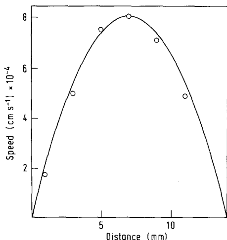
Fig. 4. Dependence of the vertical velocity of the chamber height along the z -axis. The full line shows the parabolic curve that fits best to the measured points. Polystyrene beads of 8\text{ }\mu\text{m} diameter in 0.1\text{ M NaCl} , E-field 7.6\text{ V/cm} , B-field 55 \times 10^{-4}\text{ T}
