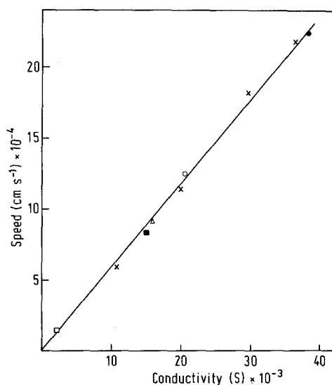
Fig. 8. Vertical velocity versus conductivity of the electrolyte. Polystyrene beads of 8\ \mu\text{m} diameter in \text{NaCl} (x), \text{HCl} (●), \text{NaOH} (○), ampholine (□); human erythrocytes in \text{NaCl} (■); Ag-suspension in \text{Na}_2\text{SO}_4 (△). E-field 7.6\ \text{V/cm} , B-field 56 \times 10^{-4}\ \text{T}
